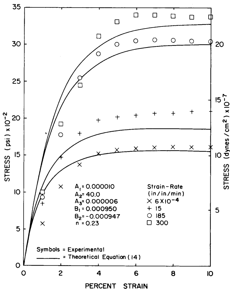
Fig. 8. Comparison between BKZ model and experimental data for polyester: A_1 in (\text{psi})^{-1} , A_2 nondimensional, A_3 in (\text{psi})^{-1} , B_1 in (\text{psi}/\text{min}^n)^{-1} , B_2 in (\text{psi}/\text{min}^n)^{-1} , n nondimensional.
